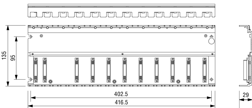
■ Basic/expansion base unit (BU668) (Unit:mm)
