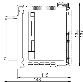
■ G2 I/O module terminal block type (Unit:mm)
