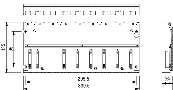
■ Basic/expansion base unit (BU668) (Unit:mm)
